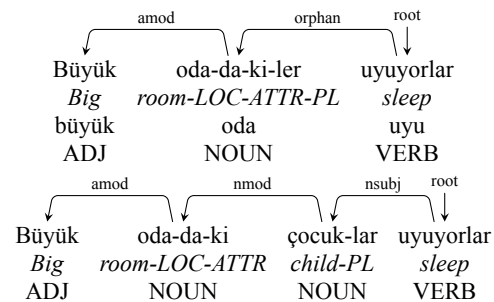
Figure 2: Analyzing -ki with no segmentation.
